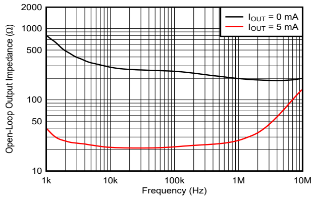
图 5-7. Open-Loop Output Impedance vs Frequency
