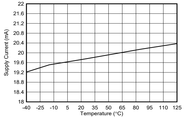
图 6-10. Supply Current vs. Temperature, Output High
