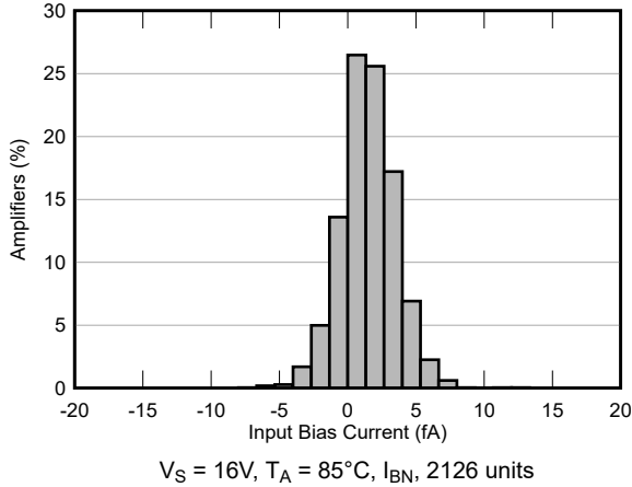
图 5-3. Input Bias Current Production Distribution
