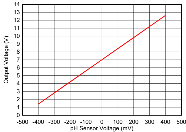
图 7-9. Single Supply, pH-Probe Sensor Transfer Function
