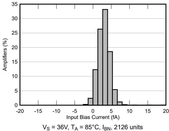
图 5-5. Input Bias Current Production Distribution
