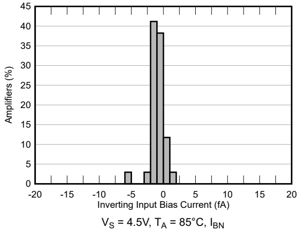
图 5-1. Input Bias Current Production Distribution
