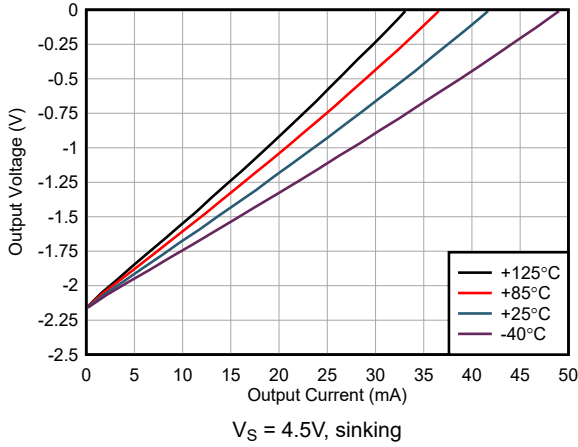
图 5-33. Output Voltage Swing vs Output Current
