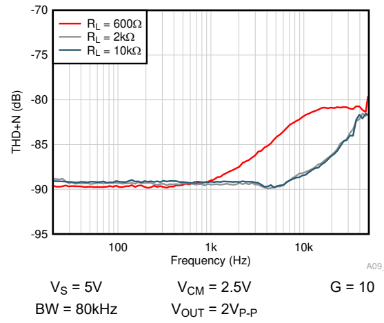
图 6-38. THD + N vs Frequency
