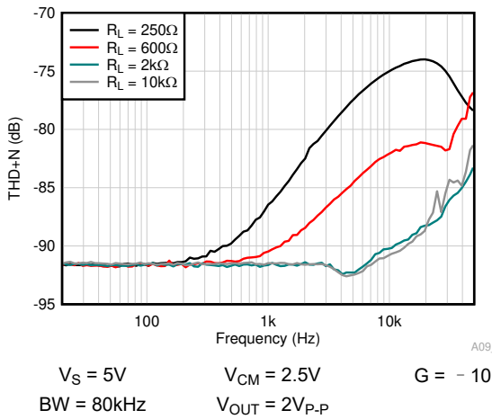
图 6-39. THD + N vs Frequency
