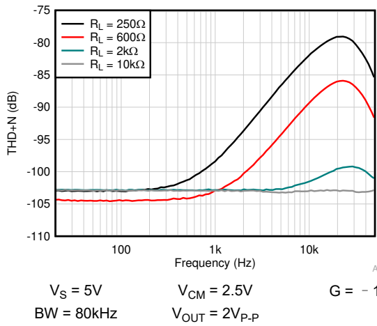
图 6-37. THD + N vs Frequency
