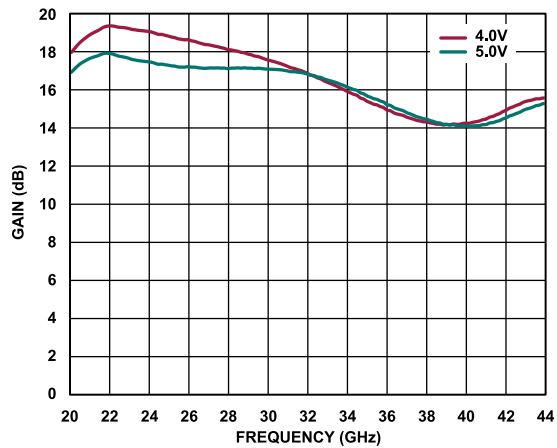
Figure 11. Gain vs. Frequency for Various Drain Voltages
