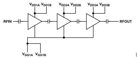
Figure 55. Simplified Internal ADPA7002CHIP Block Diagram
